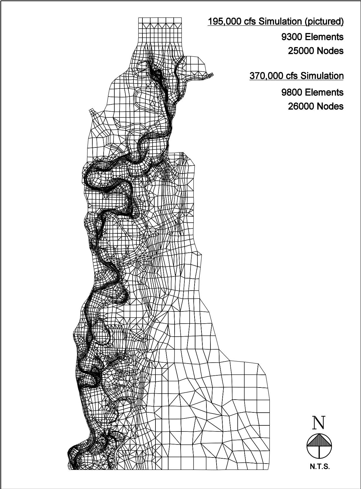
Figure 3. Finite Element Mesh
