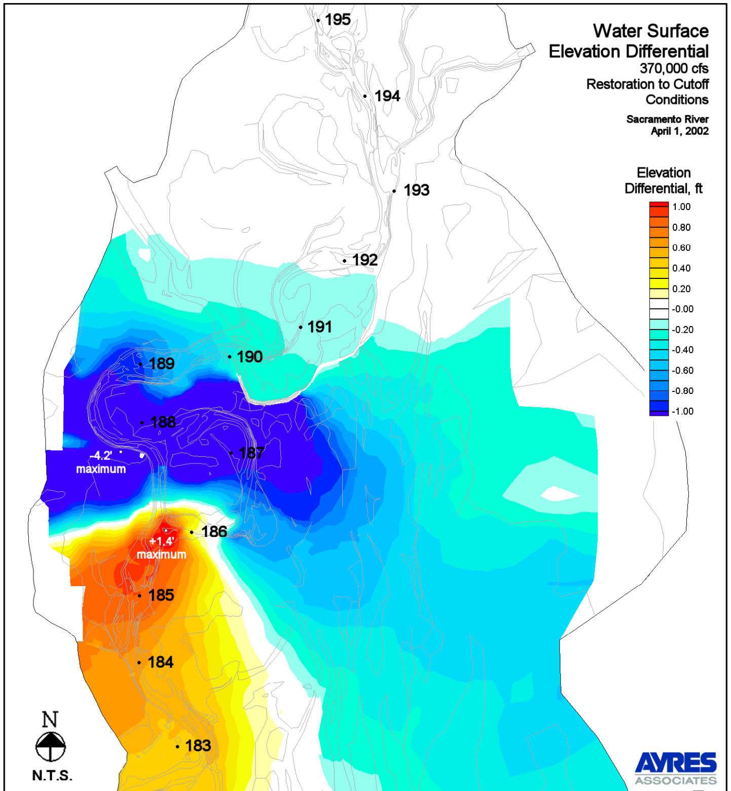
Figure 26. Water Surface Elevation Differential - Restoration to Cutoff Conditions - 370,000 cfs
