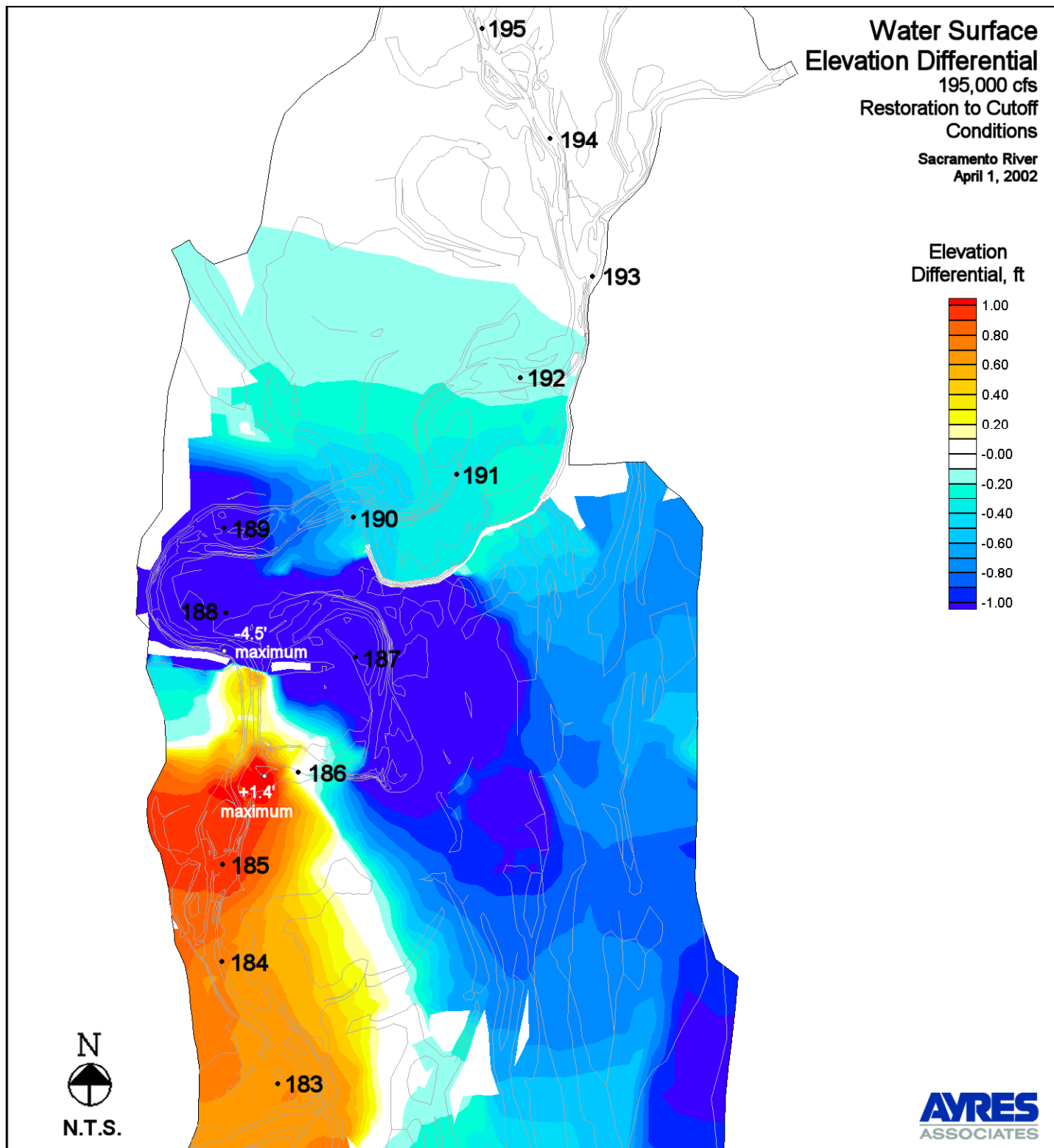
Figure 25. Water Surface Elevation Differential - Restoration to Cutoff Conditions - 195,000 cfs
