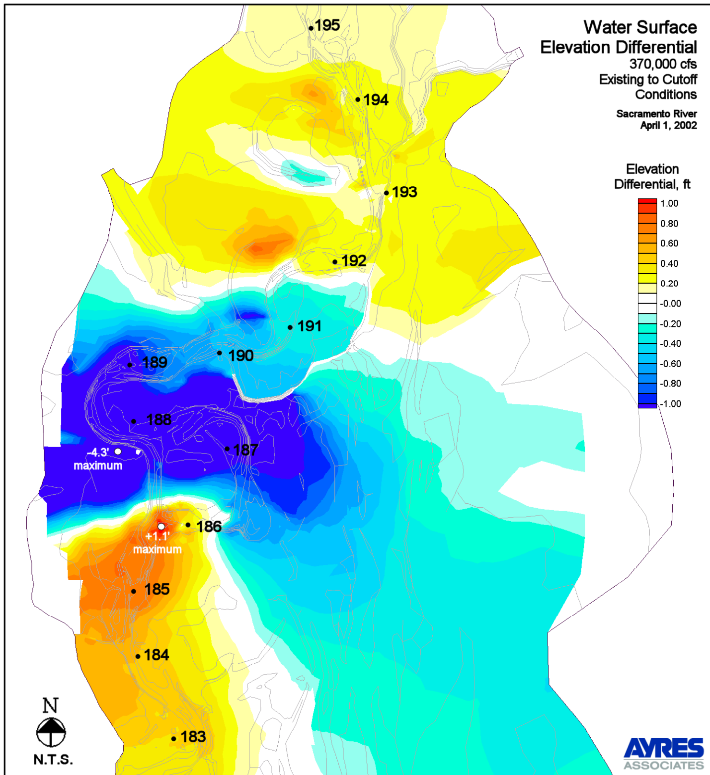
Figure 24. Water Surface Elevation Differential - Existing to Cutoff Conditions - 370,000 cfs
