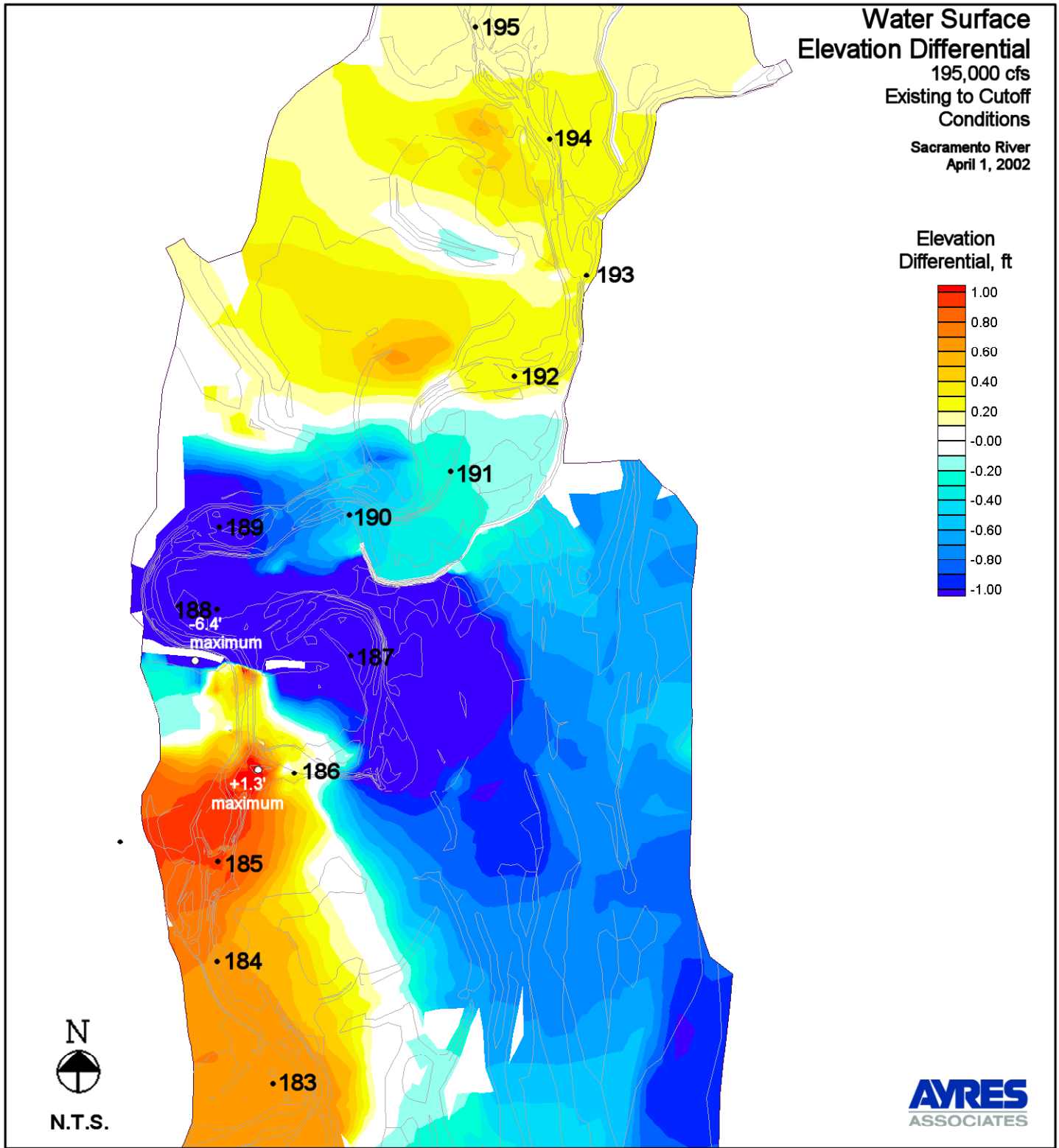
Figure 23. Water Surface Elevation Differential - Existing to Cutoff Conditions - 195,000 cfs
