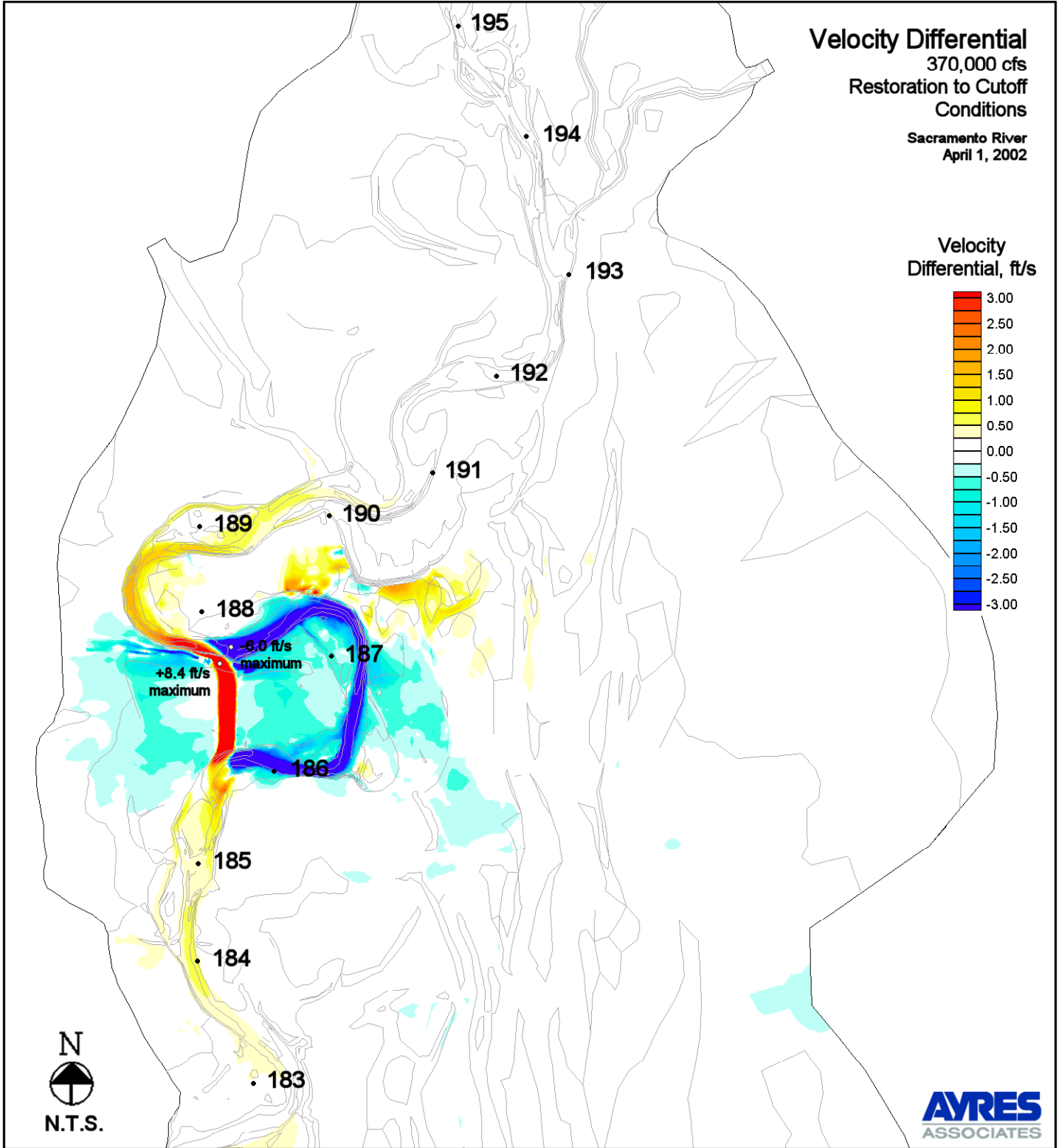
Figure 22. Velocity Differential - Restoration to Cutoff Conditions - 370,000 cfs
