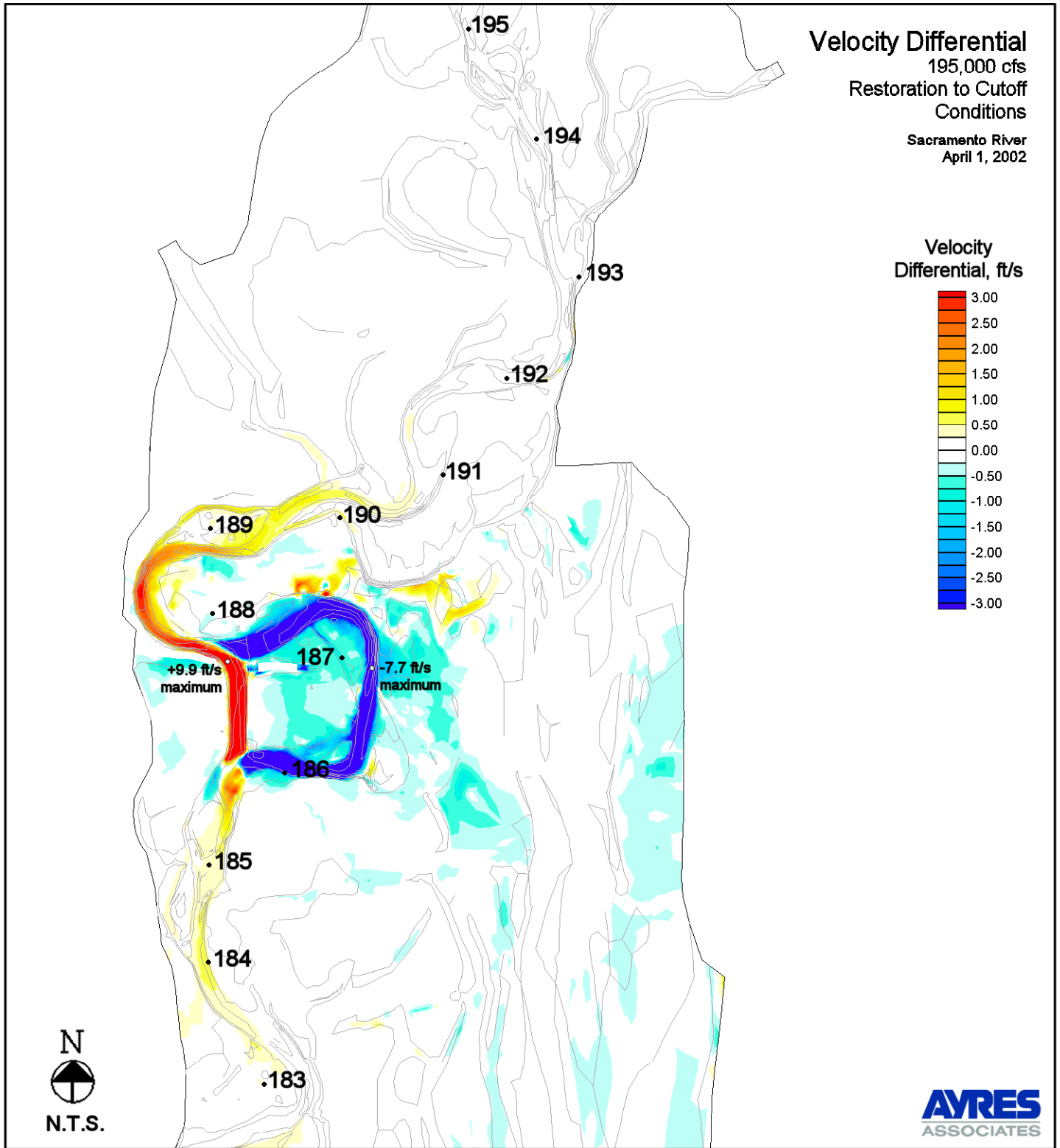
Figure 21. Velocity Differential - Restoration to Cutoff Conditions - 195,000 cfs
