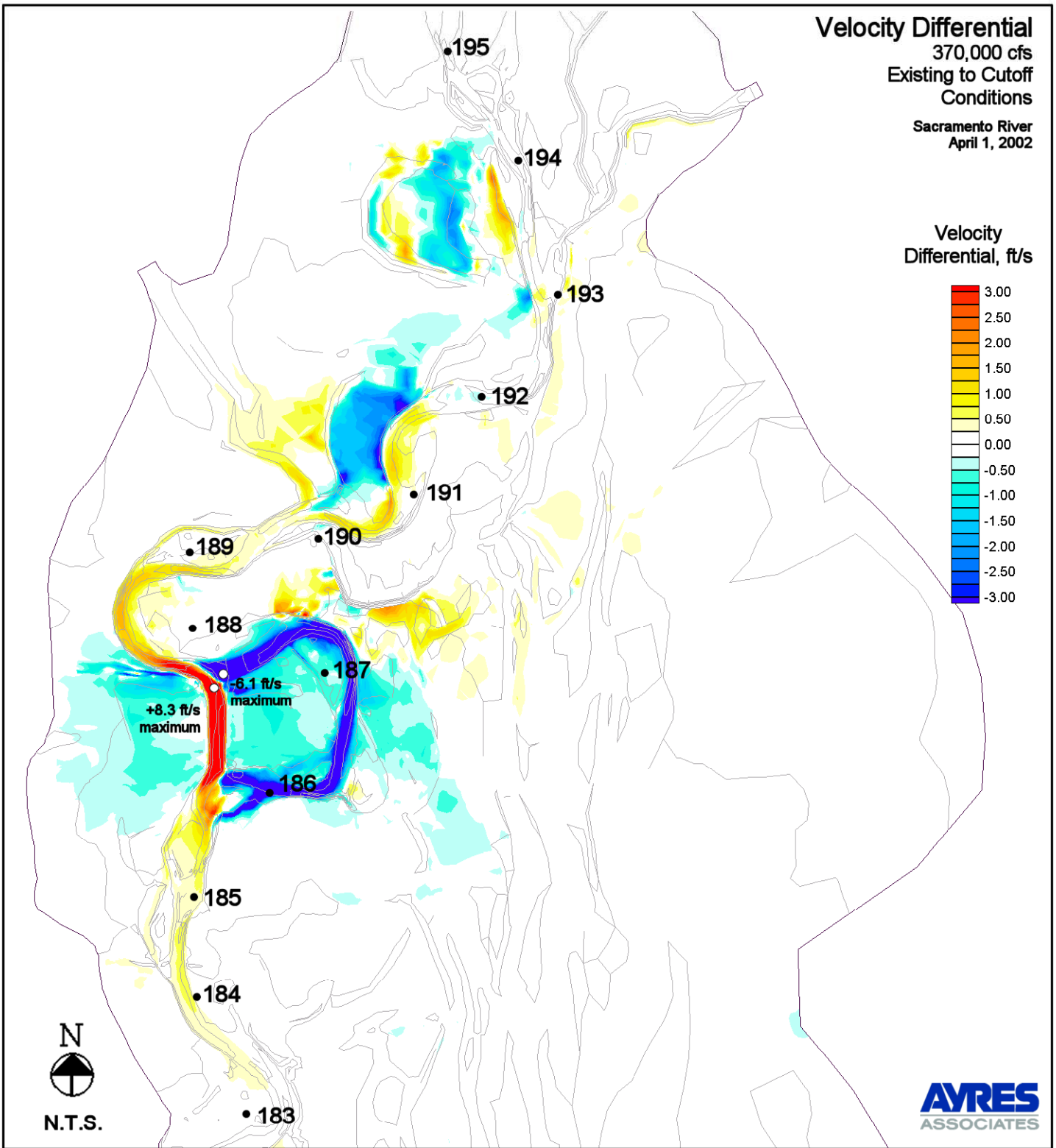
Figure 20. Velocity Differential - Existing to Cutoff Conditions - 370,000 cfs
