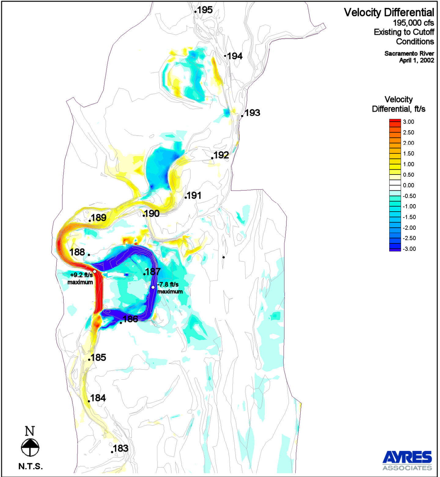
Figure 19. Velocity Differential - Existing to Cutoff Conditions - 195,000 cfs
