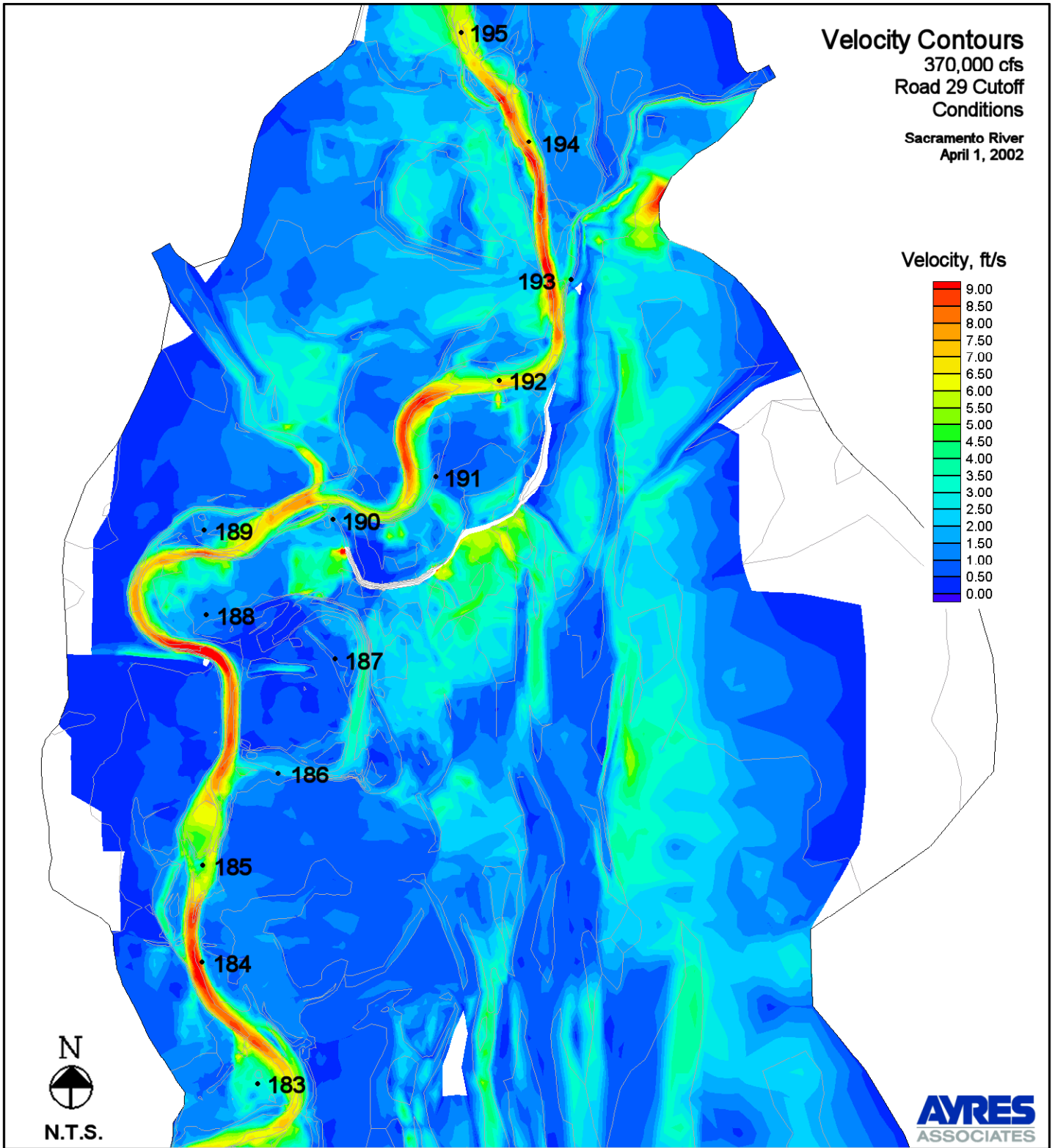
Figure 18. Velocity Contours - Road 29 Cutoff Conditions - 370,000 cfs
