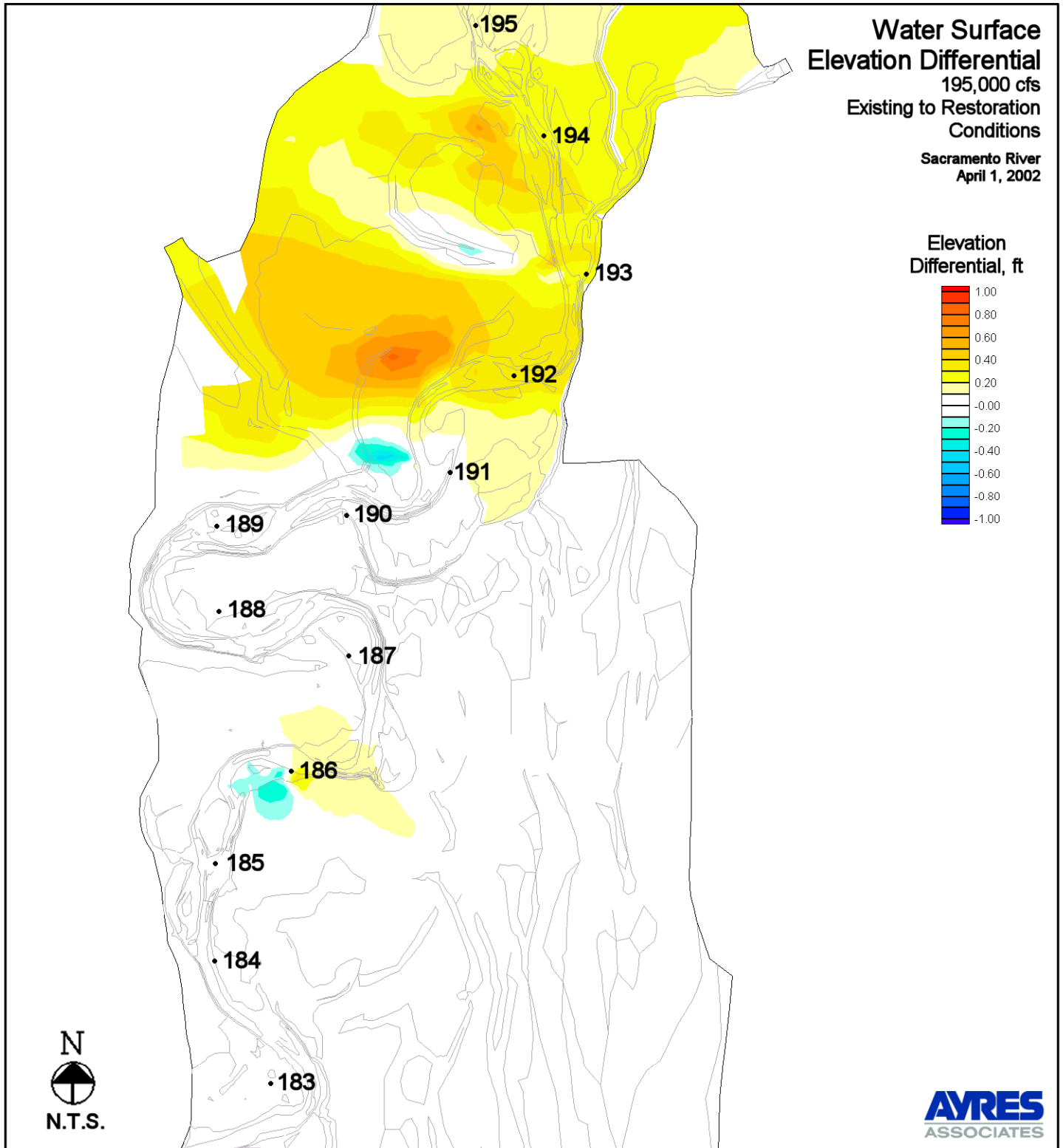
Figure 15. Water Surface Elevation Differential - Existing to Restoration Conditions, 195,000 cfs
