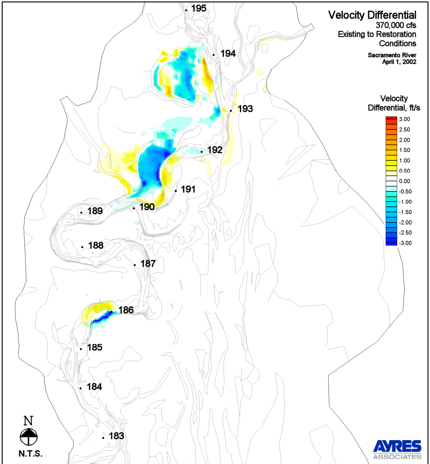
Figure 14. Velocity Differential - Existing to Restoration Conditions - 370,000 cfs
