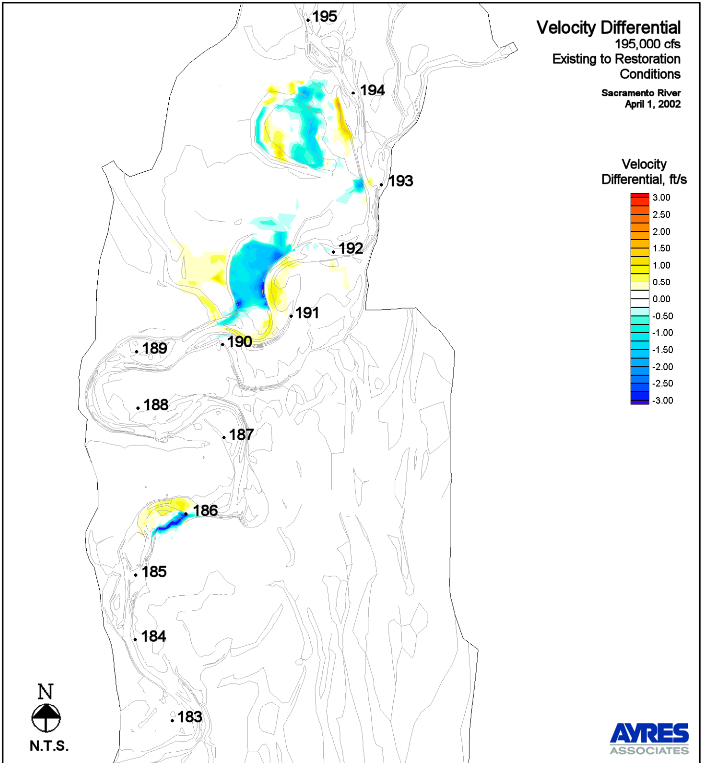
Figure 13. Velocity Differential - Existing to Restoration Conditions - 195,000 cfs
