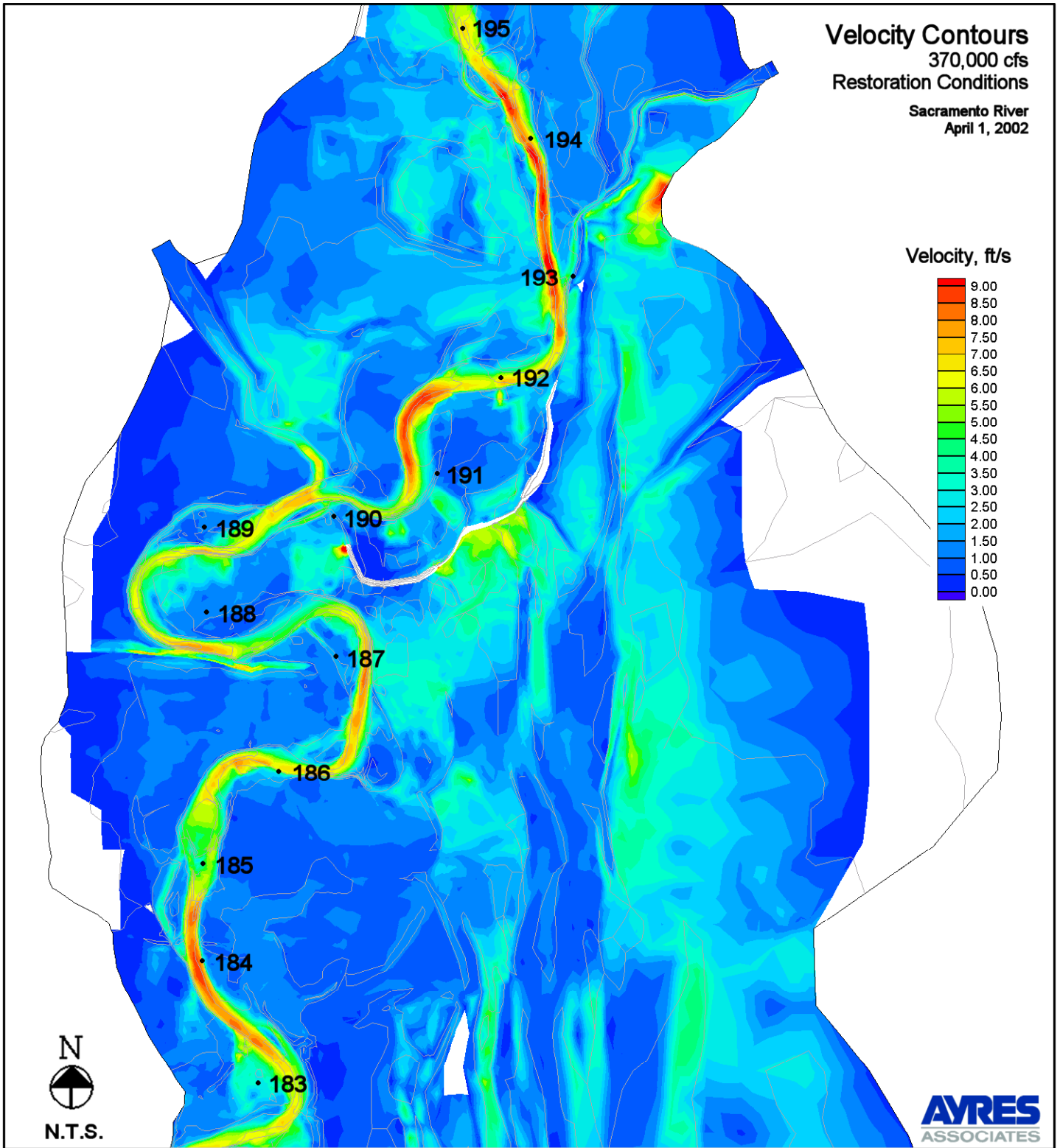
Figure 12. Velocity Contours - Restoration Conditions - 370,000 cfs
