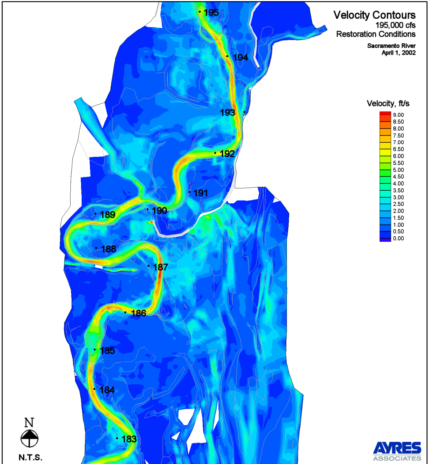
Figure 11. Velocity Contours - Restoration Conditions - 195,000 cfs
