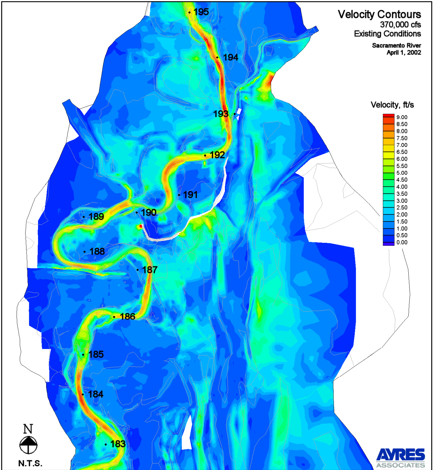
Figure 10. Velocity Contours - Existing Conditions - 370,000 cfs
