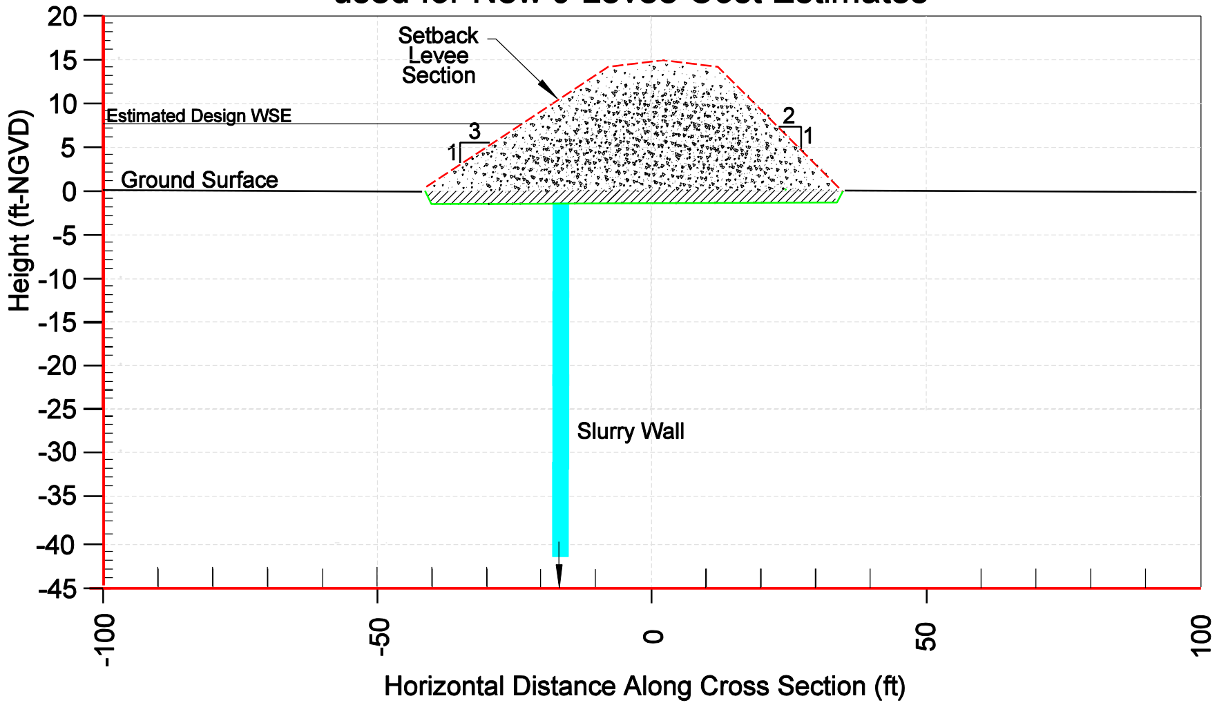
Figure 5 Typical Setback Levee Cross Section used for New J Levee Cost Estimates
