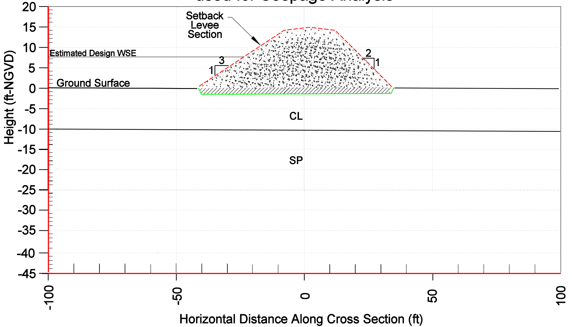
Figure 10 Setback Levee Cross Section used for Seepage Analysis
