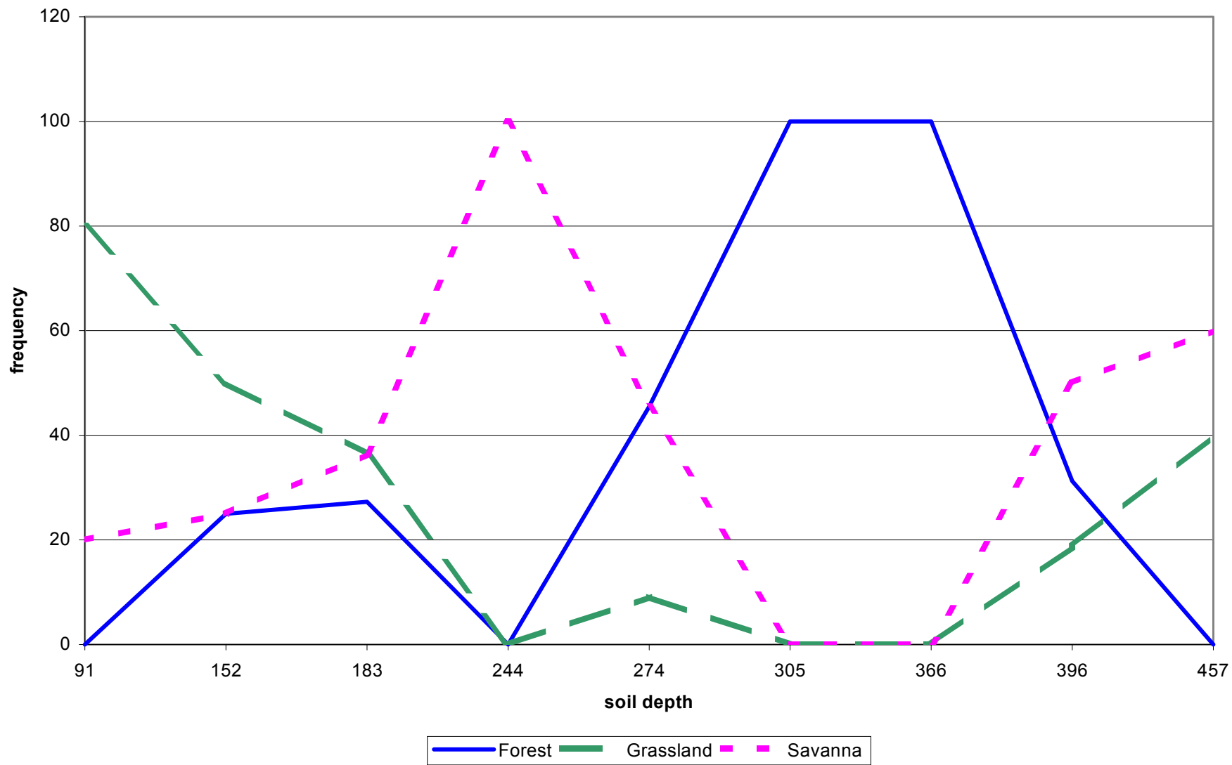
Figure 9. Frequency of vegetation cover types by soil depth
